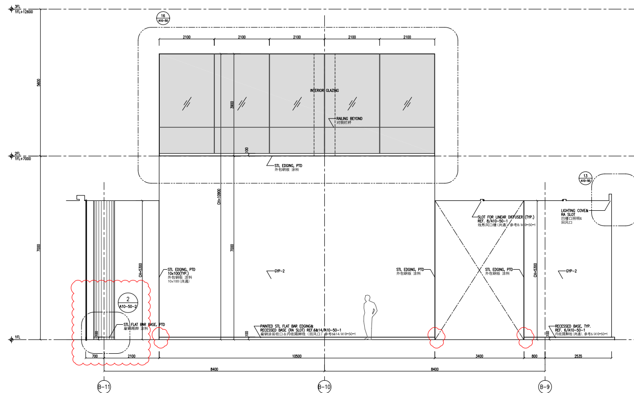
1 INTERIOR ELEVATION1
