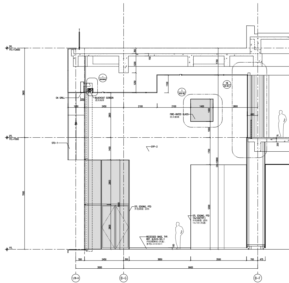
1 INTERIOR ELEVATION1
