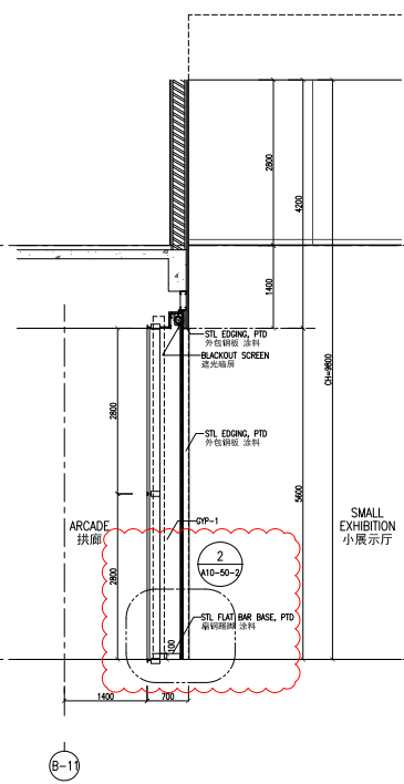
2 INTERIOR ELEVATION2
